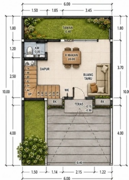
DENAH LANTAI 1
